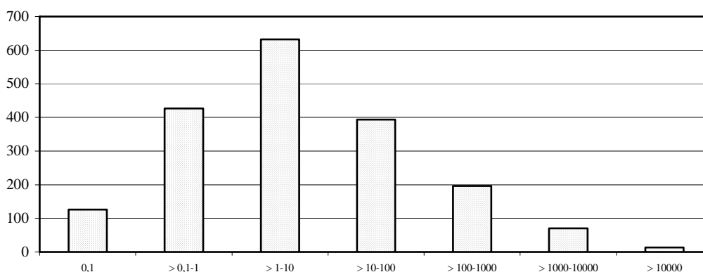
Figure 1. Number of strictly protected sites in Canada in each size range (Km 2 )
